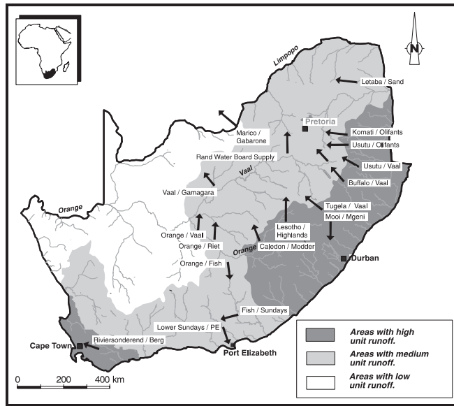
Figure 1 Major inter-basin transfer schemes in South Africa
